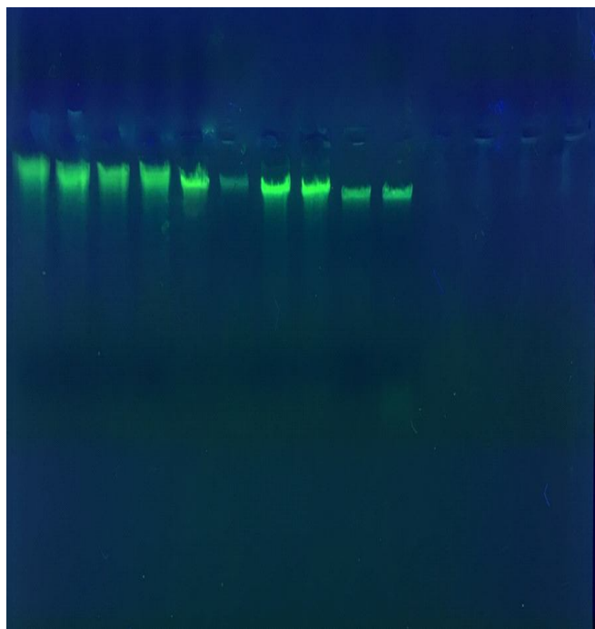
Fig. 1: Gel electrophoresis of genomic DNA extraction from P. vulgaris , DNA bands extracted using G-spin™ Total DNA Extraction Kit with 1% agarose gel, TBE buffer (1X) at 5 vol/cm for 1:15 hour.
