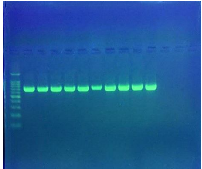
Fig. 2: PCR amplification of 16 SrRNA was electrophoresis on 2% agarose at 5 volt/cm2. 1X TBE buffer for 1:30 hours. N: DNA ladder (100),lanes (1-10),visualized under U.V light ,the band size 750 bp.
